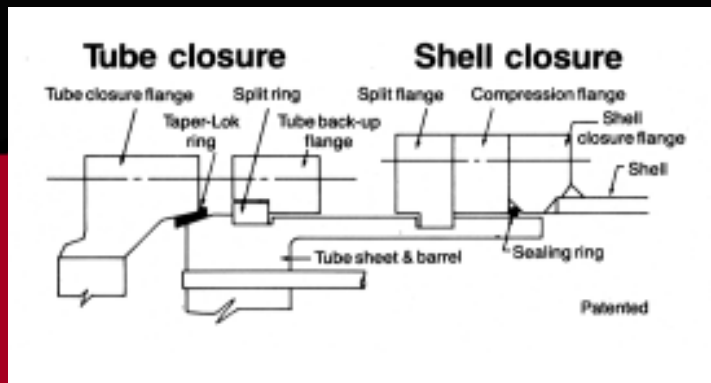
Taper-Lok® High Pressure Closure
